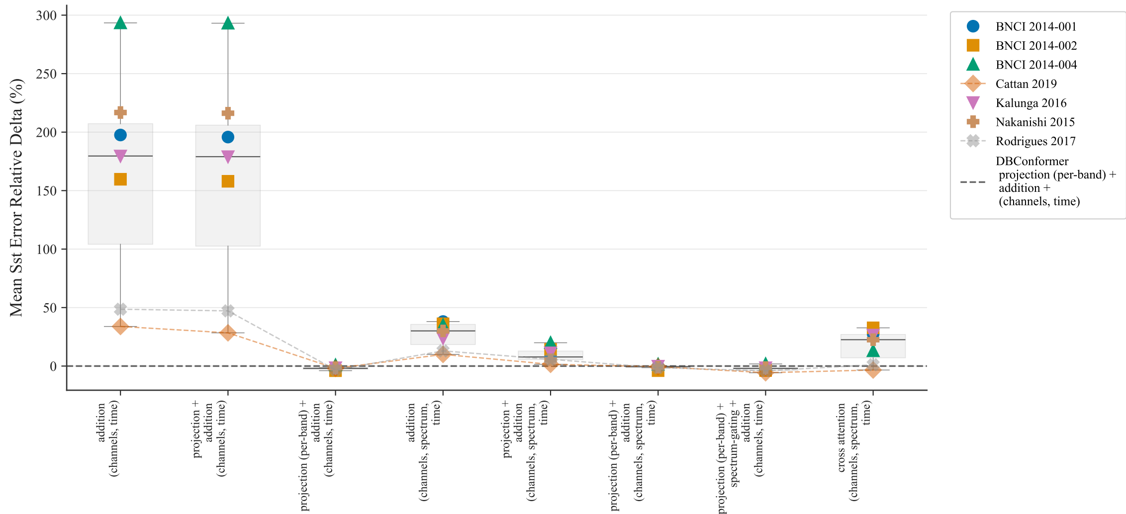
Paired Deltas by Config – Relative Delta (%)
